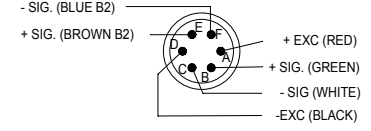
AMPHENOL PLUG
