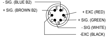
AMPHENOL PLUG
